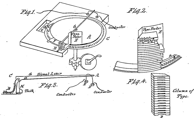
Circular Port Rule.
